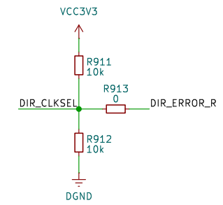
DIR Operation Mode and Clock Source
